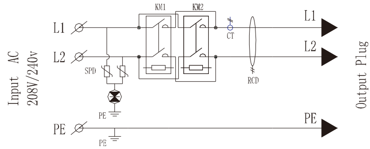
Fig14-1. Main circuit diagram
